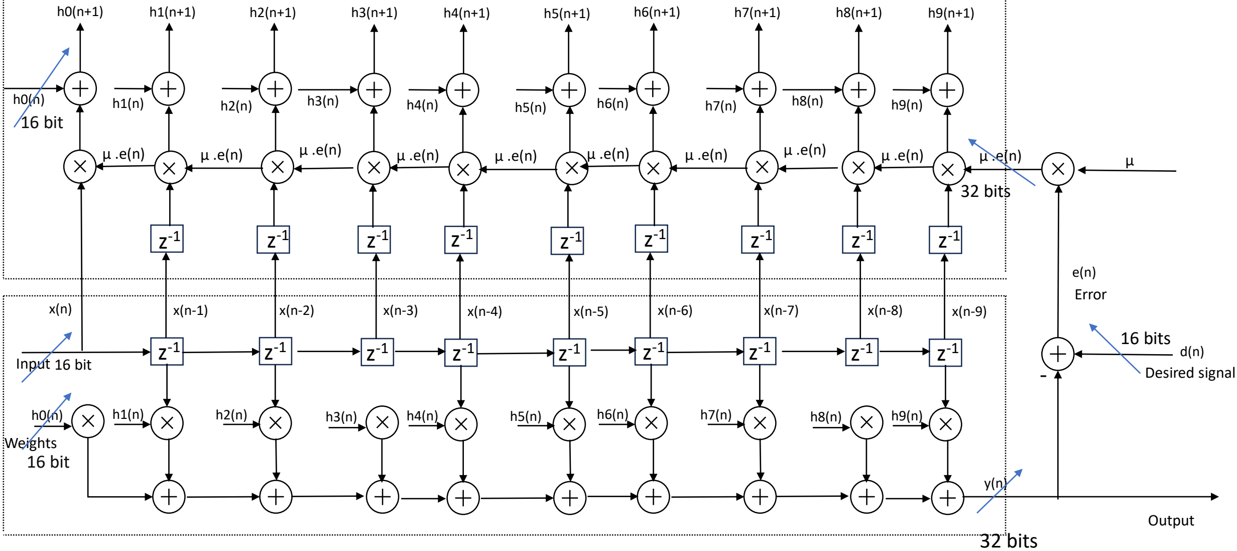
FIR Filter
